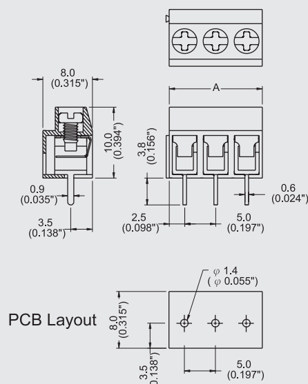
PCB Layout
