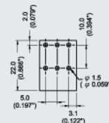
PCB Layout
