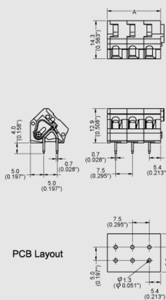
PCB Layout
